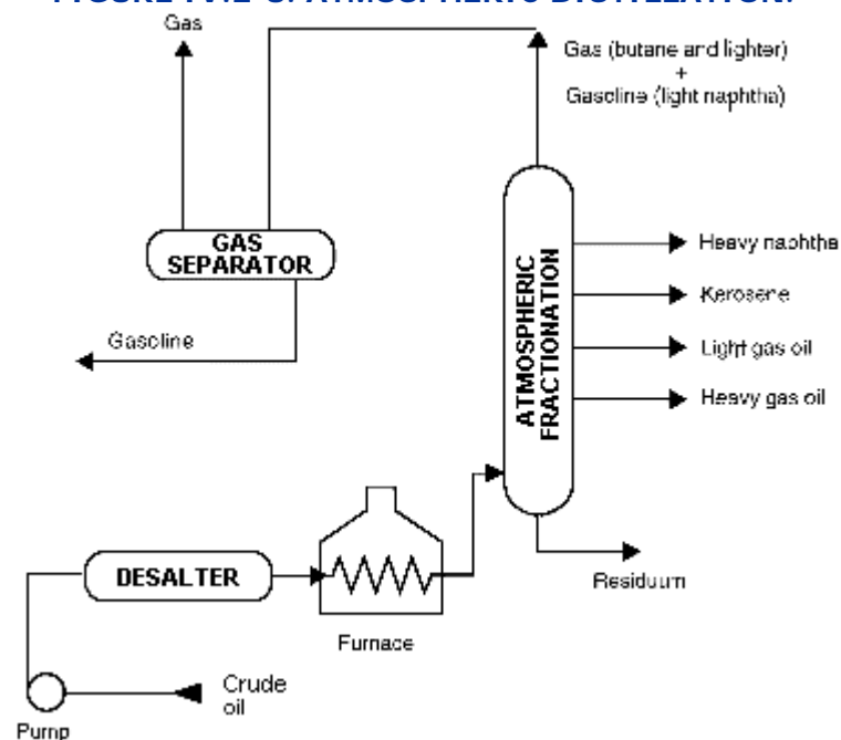
FIGURE IV:2-8. ATMOSPHERIC DISTILLATION.
