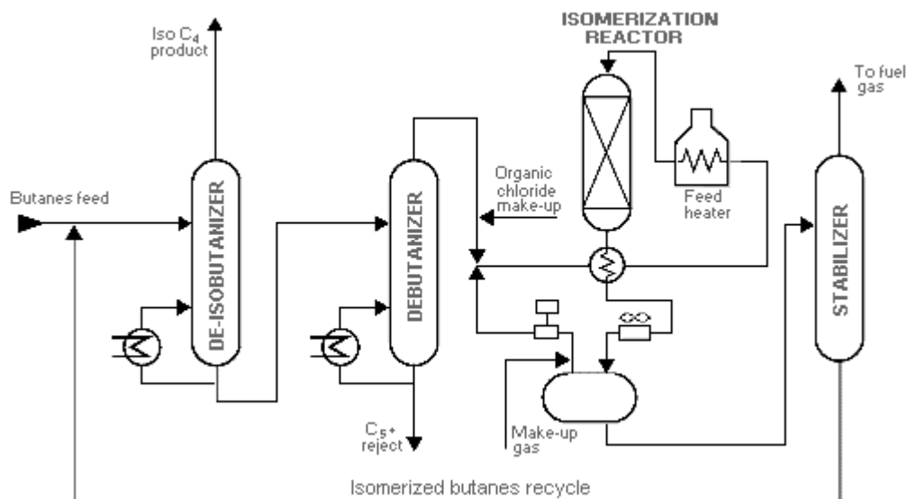
FIGURE IV:2-18. C 4 ISOMERIZATION.
