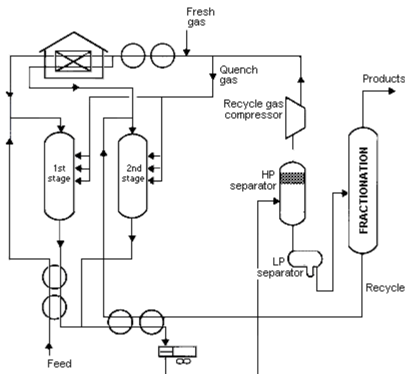
FIGURE IV:2-15. TWO-STAGE HYDROCRACKING.
