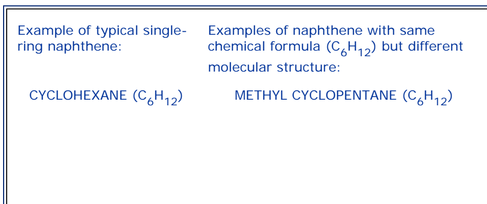
FIGURE IV:2-3. TYPICAL NAPHTHENES.
