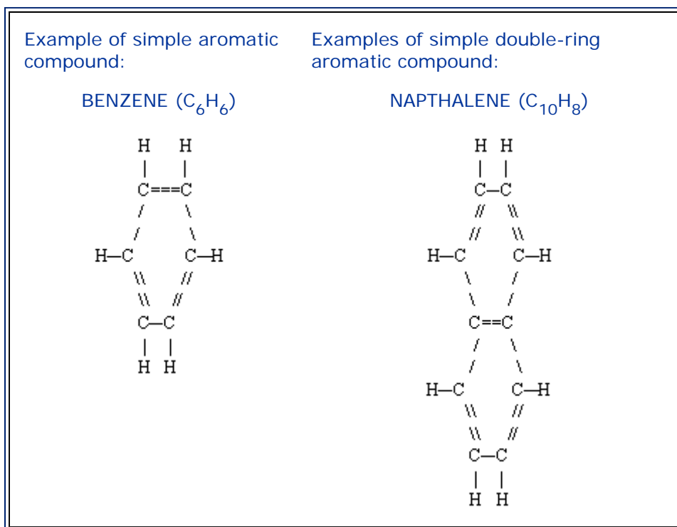
FIGURE IV:2-2. TYPICAL AROMATICS.
