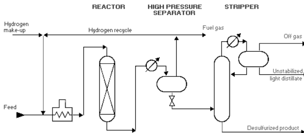
FIGURE IV:2-17. DISTILLATE HYDRODESULFURIZATION.
