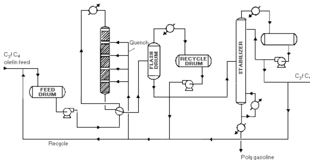
FIGURE IV:2-20. POLYMERIZATION PROCESS.
