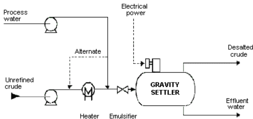
FIGURE IV:2-7. ELECTROSTATIC DESALTING.
