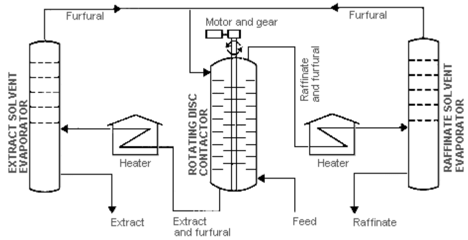
FIGURE IV:2-10. AROMATICS EXTRACTION.
