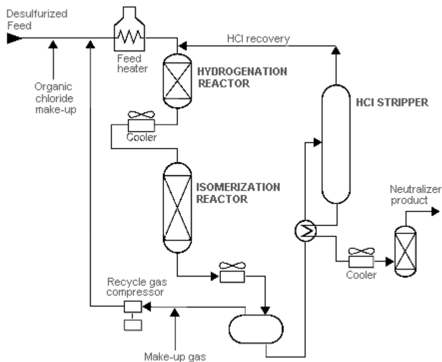
FIGURE IV:2-19. C 5 AND C 6 ISOMERIZATION.
