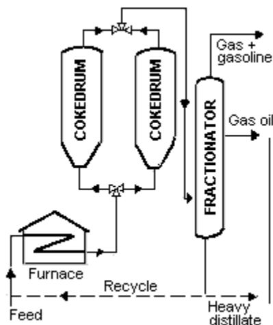
FIGURE IV:2-13. DELAYED COKING.
