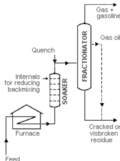
FIGURE IV:2-12. VISBREAKING.
