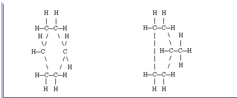
FIGURE IV:2-4. TYPICAL ALKENES.
