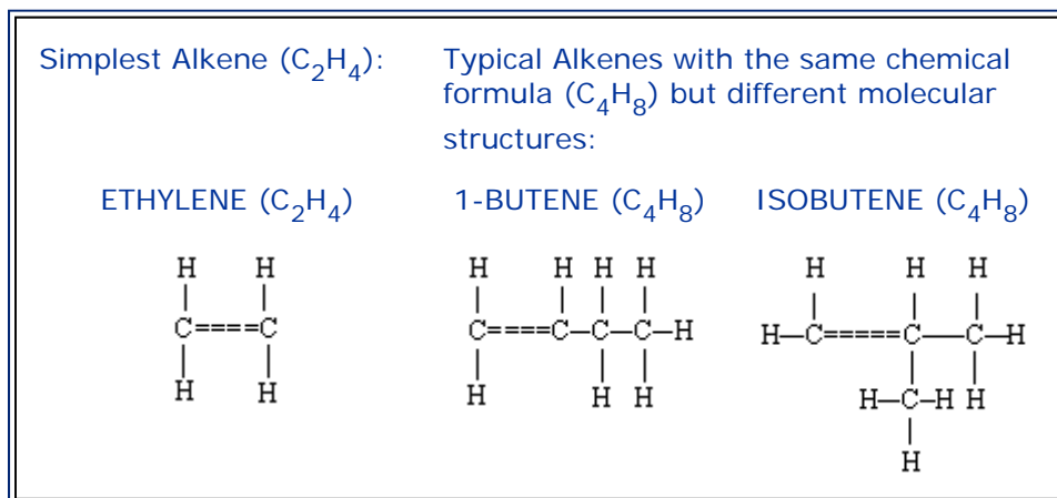
FIGURE IV:2-4. TYPICAL ALKENES.
