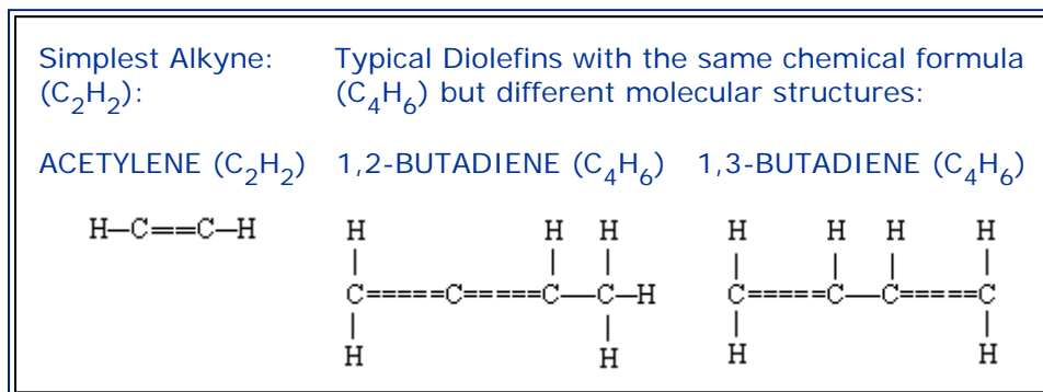
FIGURE IV:2-5. TYPICAL DIOLEFINS AND ALKYNES.
