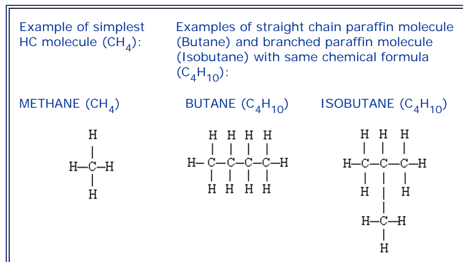
FIGURE IV:2-1. TYPICAL PARAFFINS.
