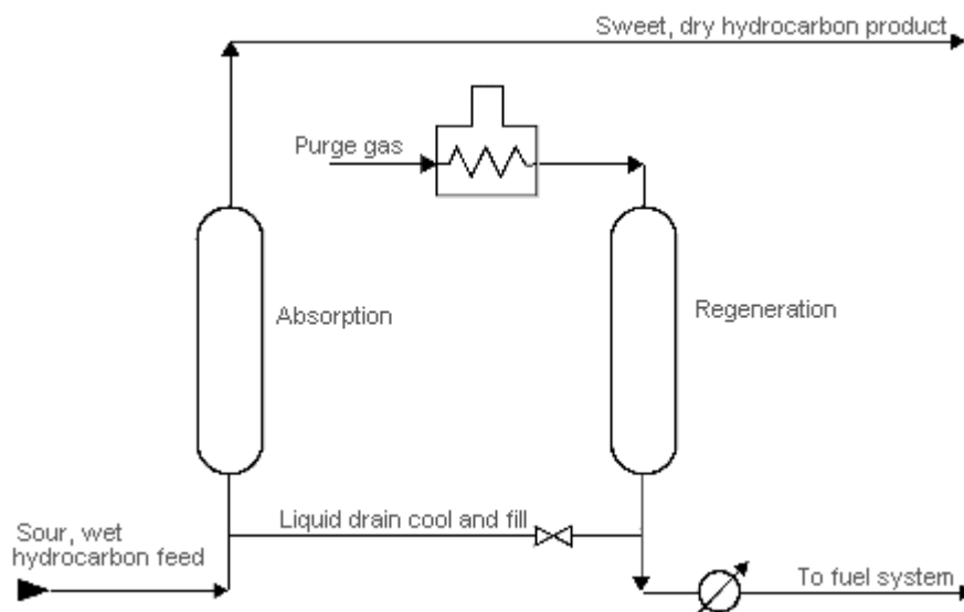
FIGURE IV:2-23. MOLECULAR SIEVE DRYING AND SWEETENING.
